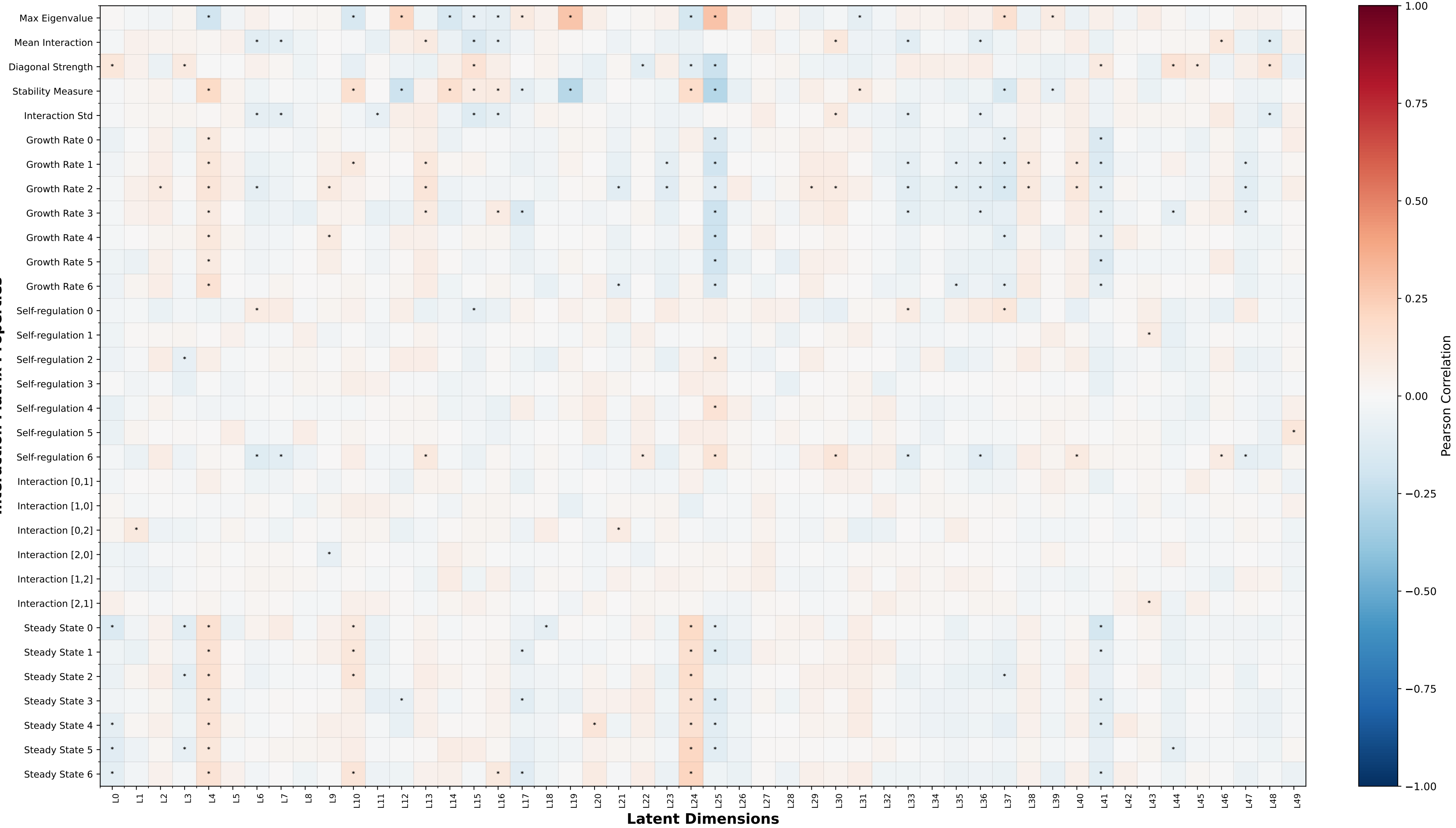
Correlation Heatmap: 50 Latent Dimensions vs GLV Properties (Pearson correlation, * indicates p<0.01)
